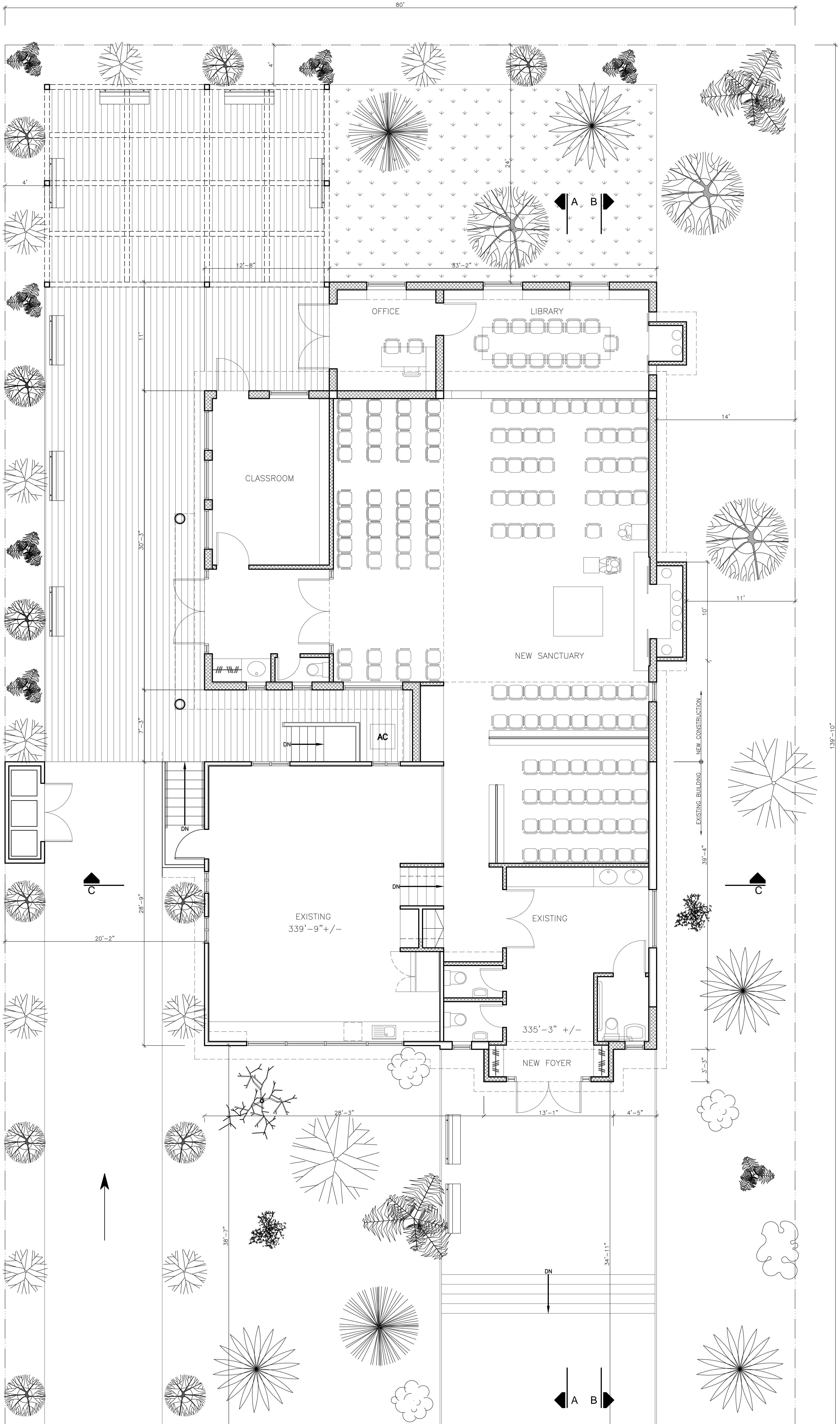
1ST FLOOR PLAN SCALE: 1/4" = 1'-0"
