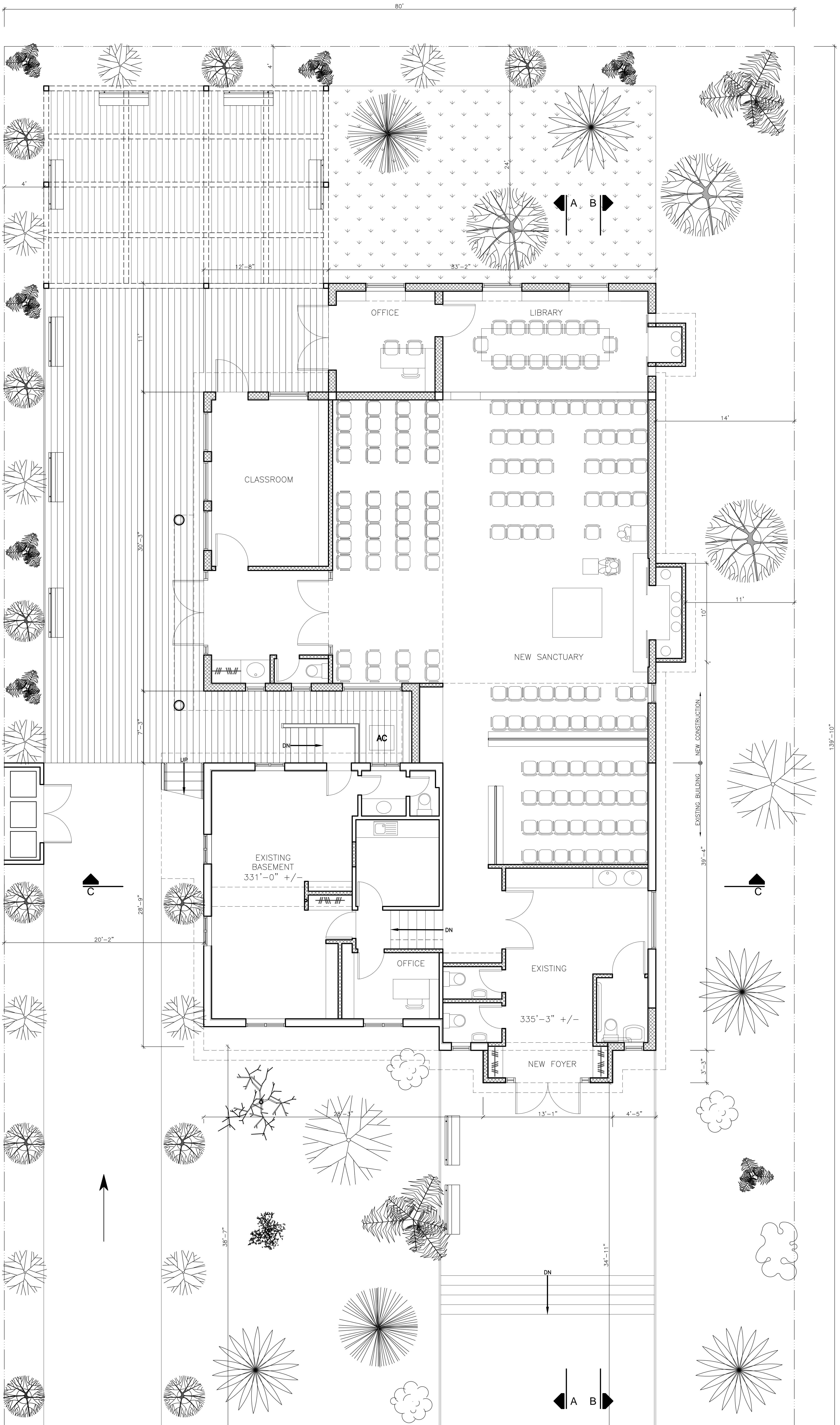
BASEMENT FLOOR PLAN SCALE: 1/4" = 1'-0"
